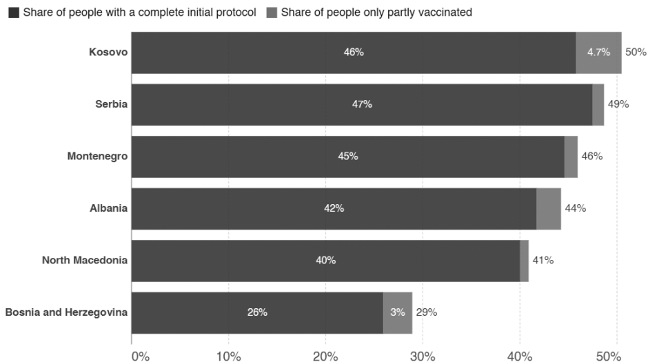
Share of people vaccinated against COVID-19, Feb 28, 2022
